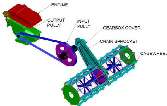
Fig. 7: Power transmission system of Hydro tiller.
