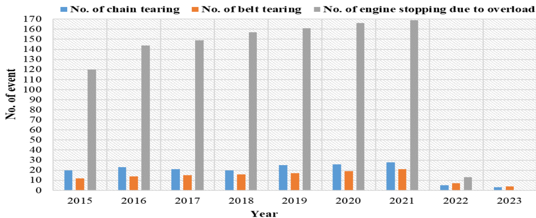
Fig. 10: Chain, belt tearing and engine stopping scenario of the hydro-tiller.
