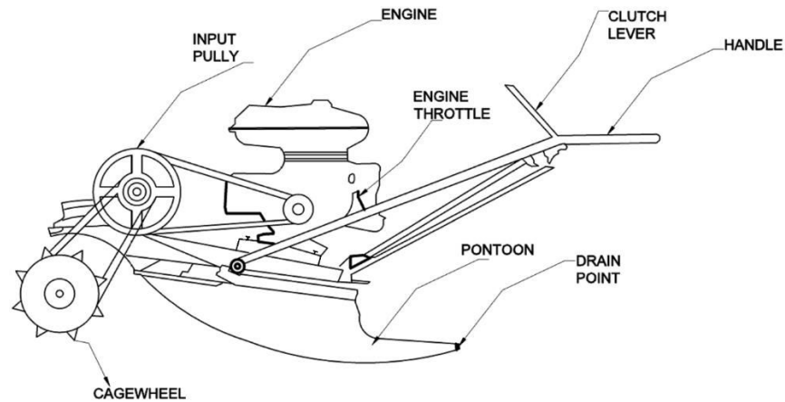
Fig. 5: A schematic diagram of the modified Hydro tiller.
