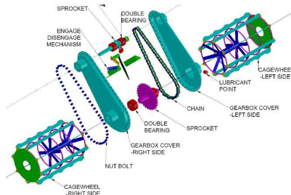
Fig. 8: Exploded view of power transmission system between gearbox and cage wheel
